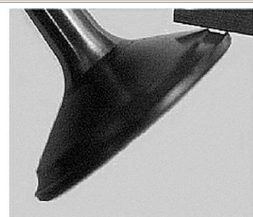
Worn valve face
